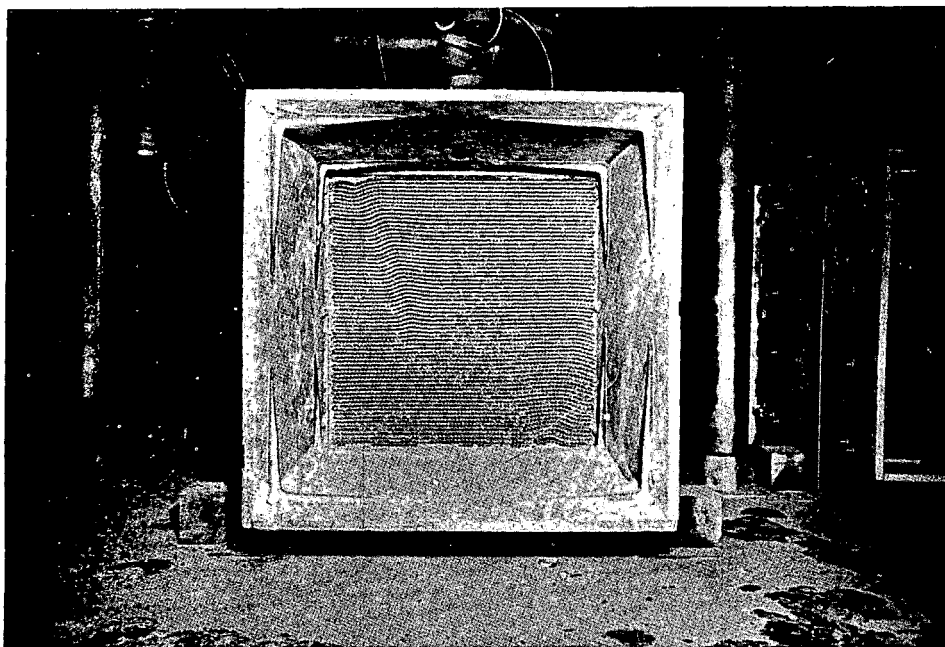
Fig. 12—Dust loss from 12-in. AEC filter in hood 4 in chemical plant, postshot.
